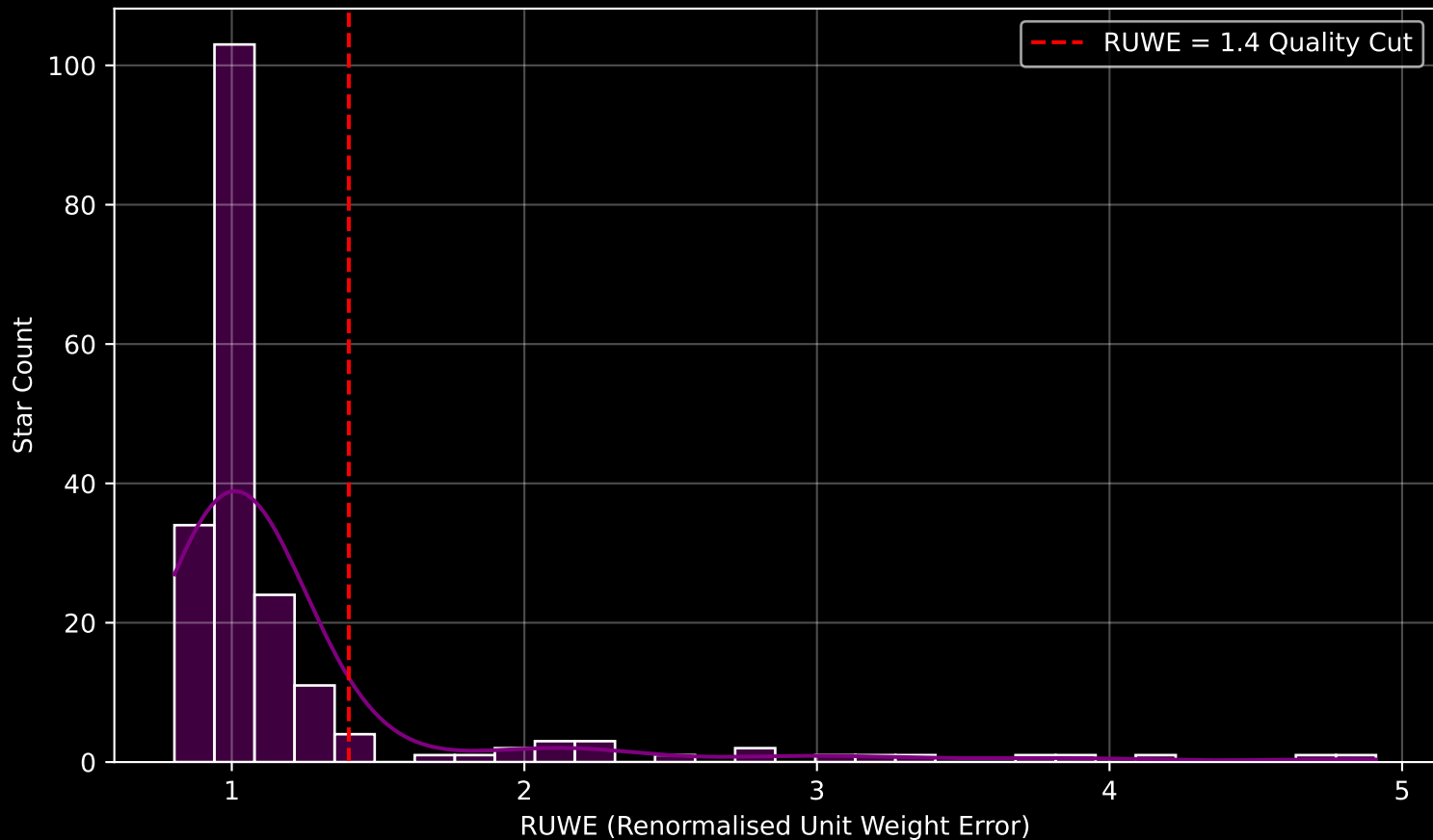
GAPOGEE DR17 Field [K2_C8_133-60] RUWE Distribution (n= 197)
