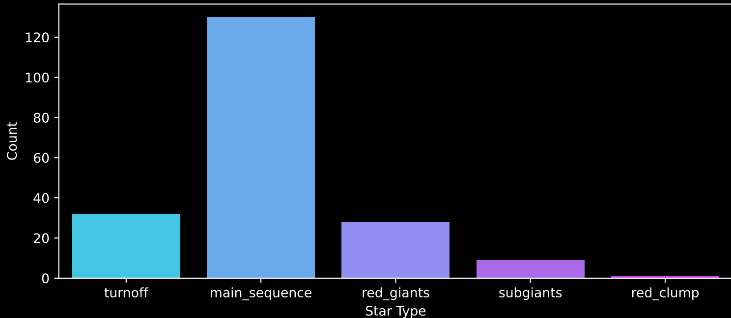
APOGEE DR17 Field: [K2_C8_133-60] Count plot of Star Type
