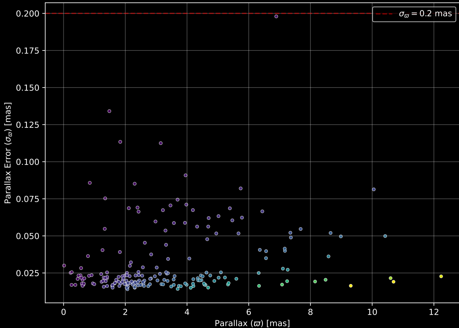
APOGEE DR17 Field: [K2_C8_133-60] Parallax Quality (n= 200)
