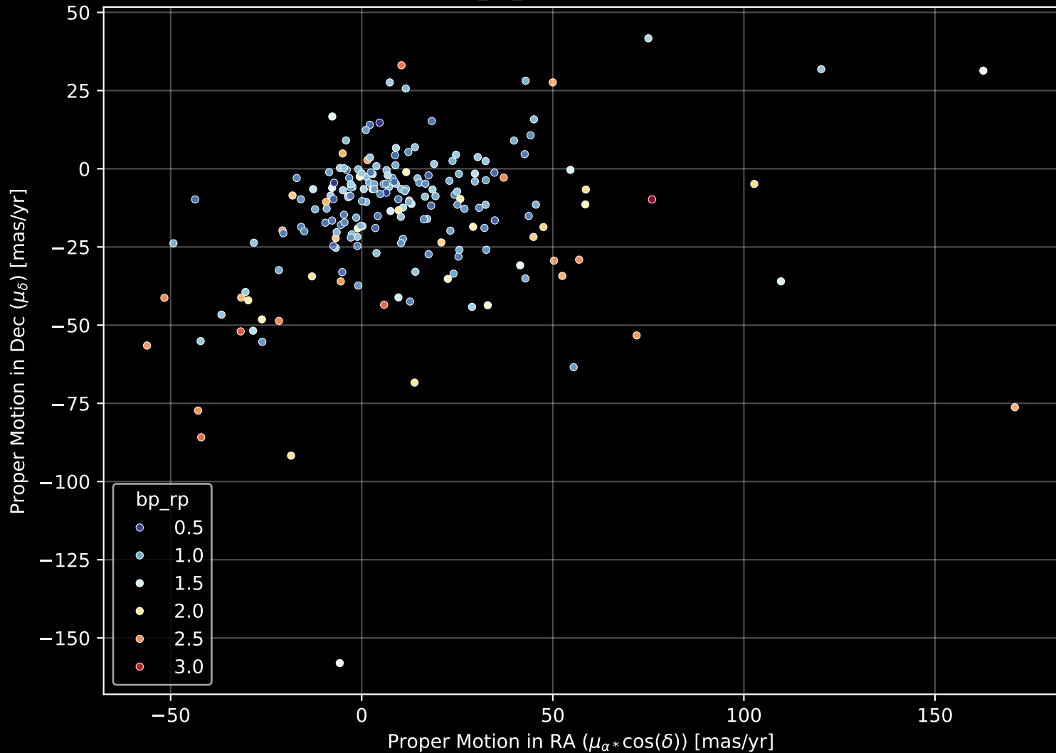
APOGEE DR17 Field: [K2_C8_133-60] Proper Motion Diagram (n= 200)
