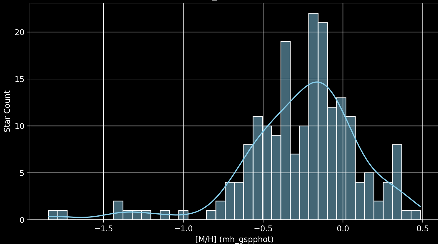
APOGEE DR17 Field: [K2_C8_133-60 [M/H] (mh_gspphot) (n= 198)
