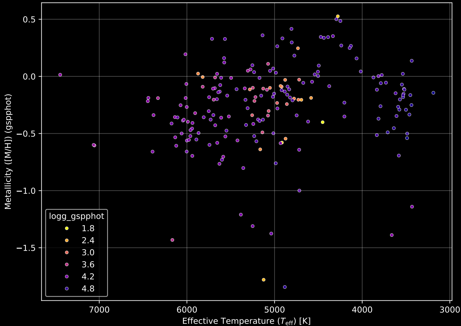
APOGEE DR17 Field: [K2_C8_133-60] Stellar Population Parameters (n= 200)
