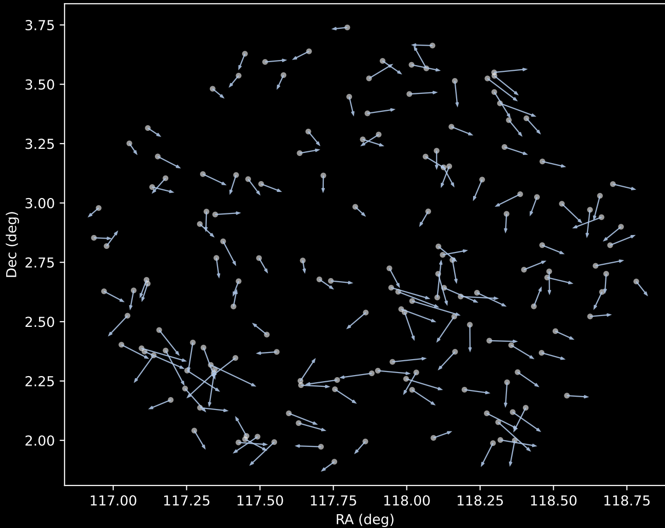
APOGEE DR17 Cluster 1 Proper Motion Vectors (n=159)
